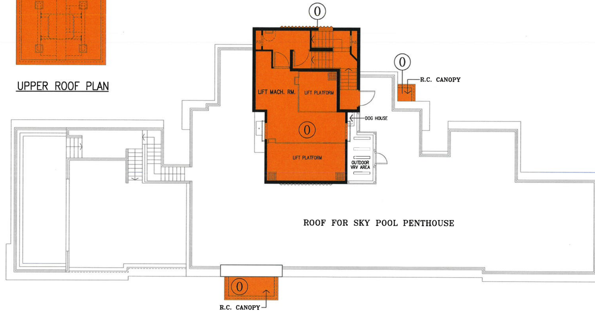
ROOF PLAN
