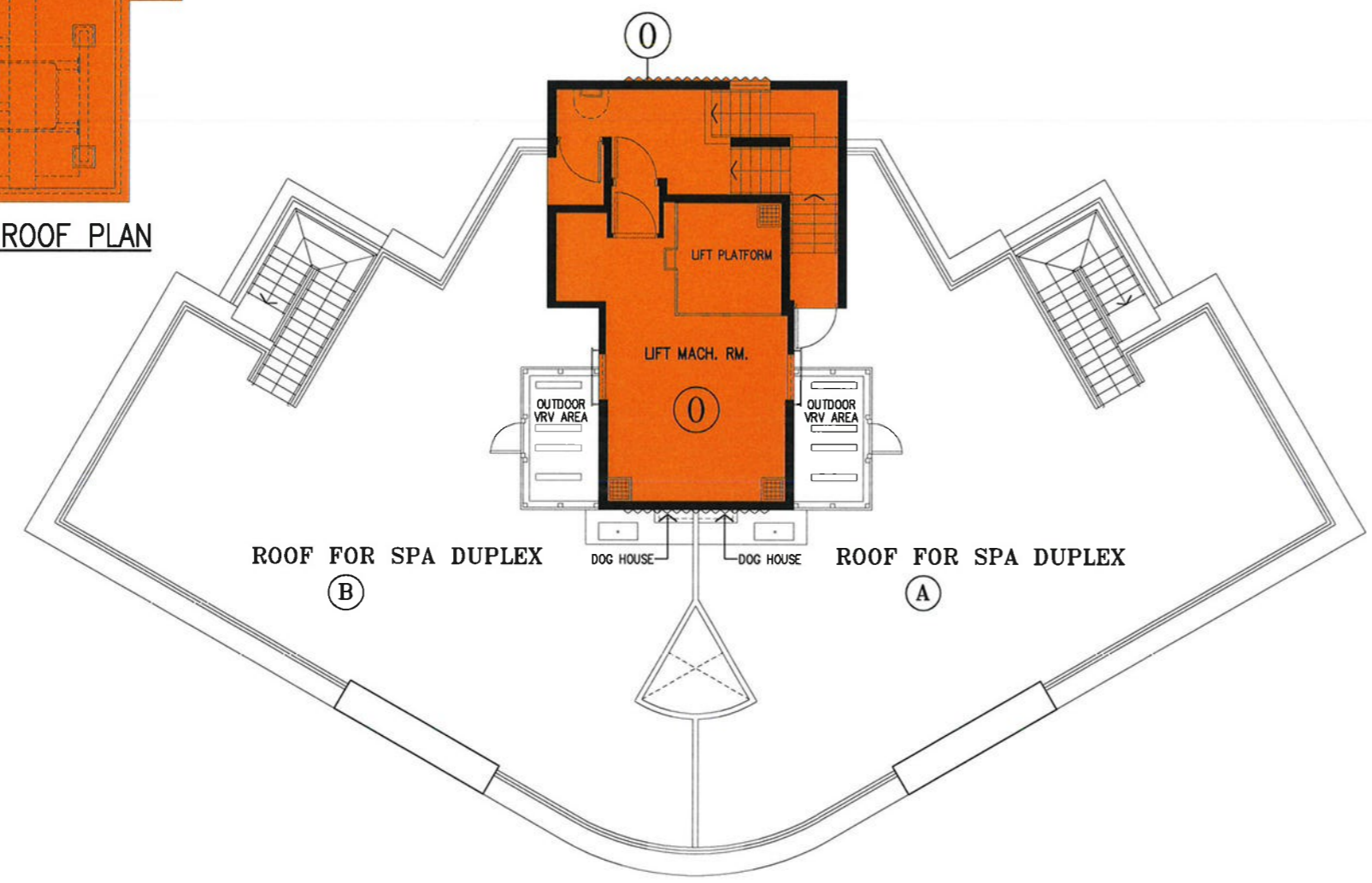
ROOF PLAN
